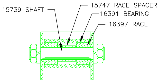
DETAIL "D"
