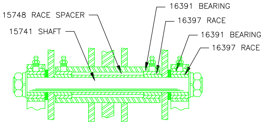
DETAIL "A"
